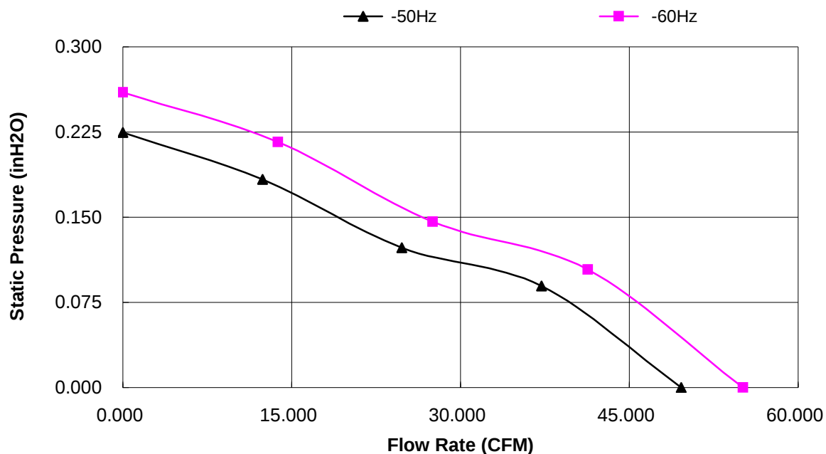
Fan Performance Curve
